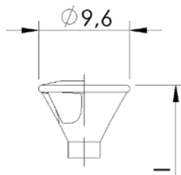
Flat countersunk head 60° / 75°, with and without raised head, with and without milling pockets
