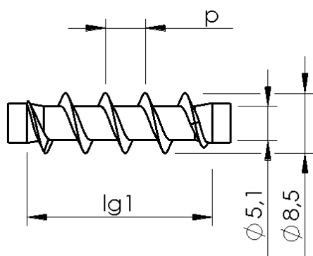
Secondary thread
