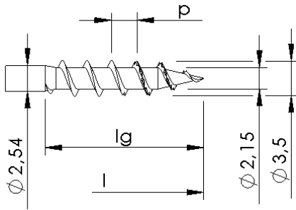
With and without variation, with toothed tip
