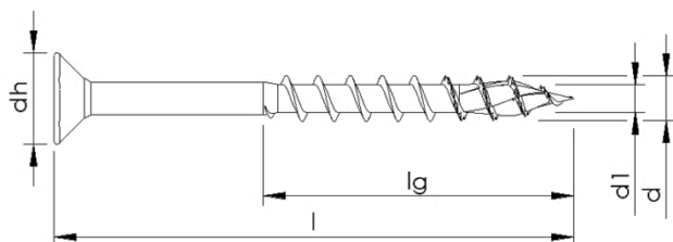
Part thread without variation, without shank ribs, with toothed tip and milling ribs
