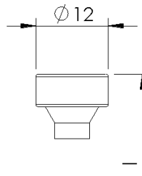
Cylindrical head with counter-sinking
