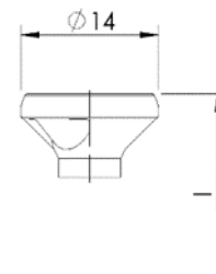
Flat countersunk head 90°, with and without milling pockets
