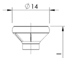
Flat countersunk head 90°, with and without milling ribs
