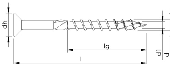
Part thread without variation, with shank ribs, with toothed tip and milling ribs
