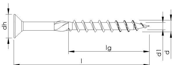
Part thread without variation, with shank ribs and toothed tip
