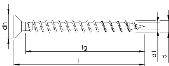
Full thread with variation, toothed tip
